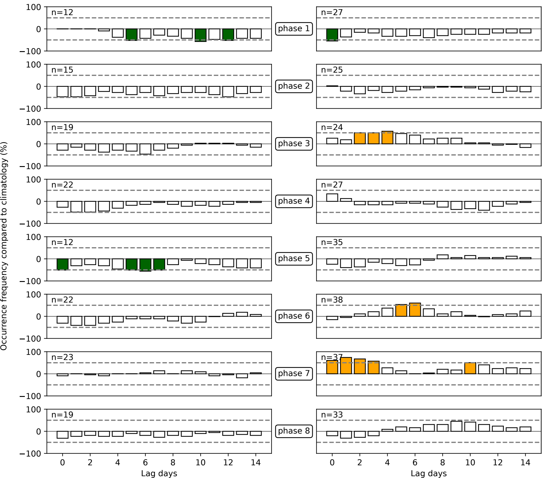
(a) BSISO
