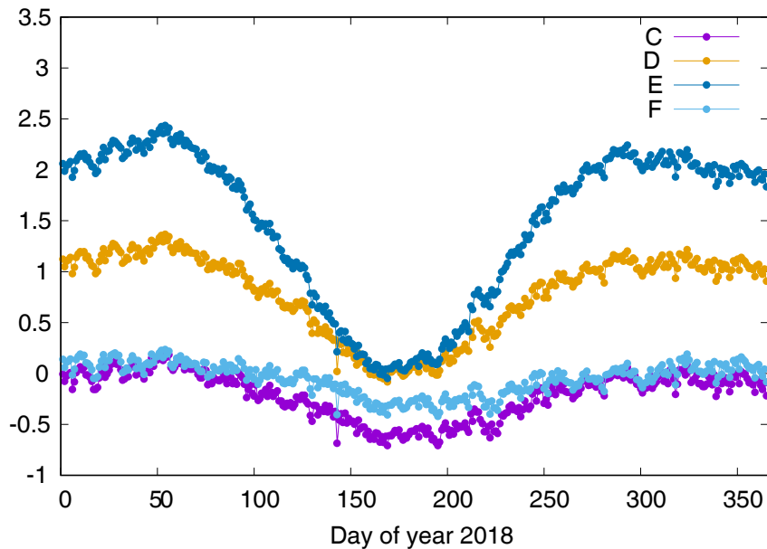
(a) Sentinel-1A
