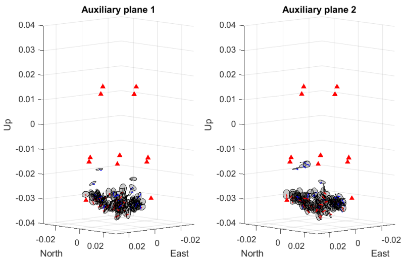
(b) Fault planes at bottom of sample
