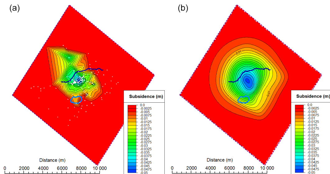
Figure 5. Comparison of surface deformation between measured data (a) and history match result (b) for 2009–2013 – white dots in the left plot show the locations of the measurement points.
