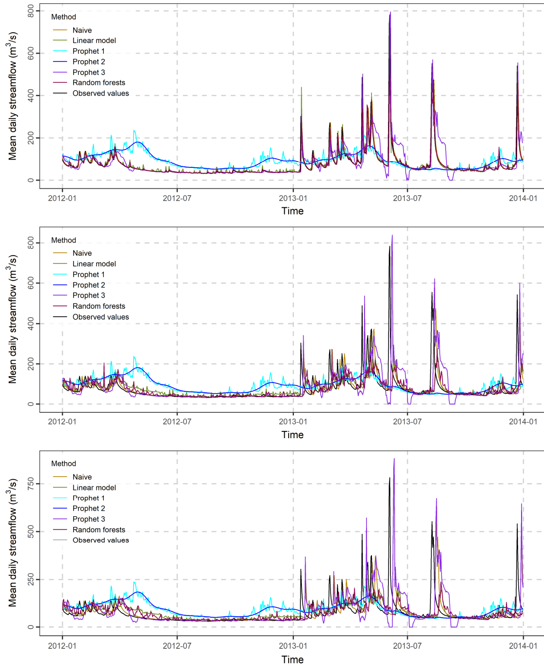
Figure S.2. 1-, 4- and 7-step ahead forecasts (from top to bottom) of the Current river daily streamflow in the period 2012-2013.
